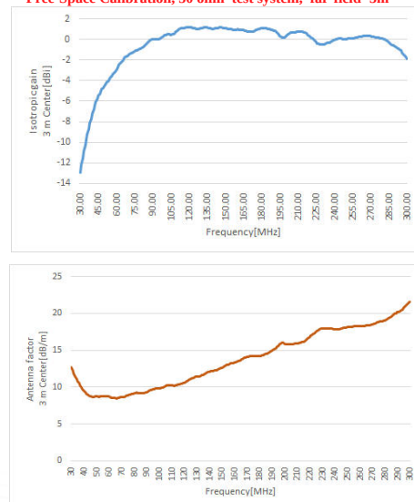
Free-Space Calibration, 50 ohm test system, far-field=3m
