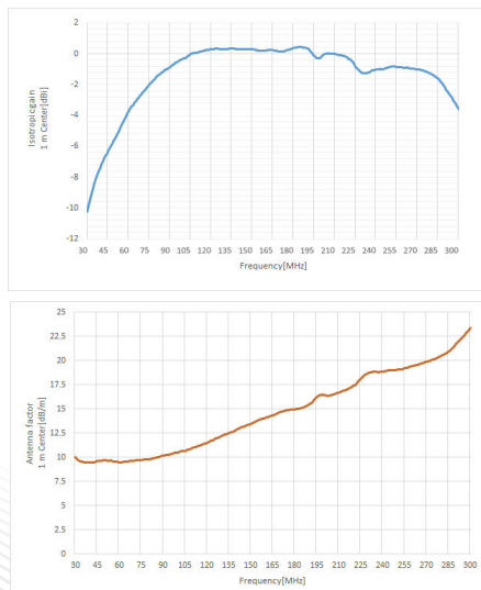
Free-Space Calibration, 50 ohm test system, far-field=1m
